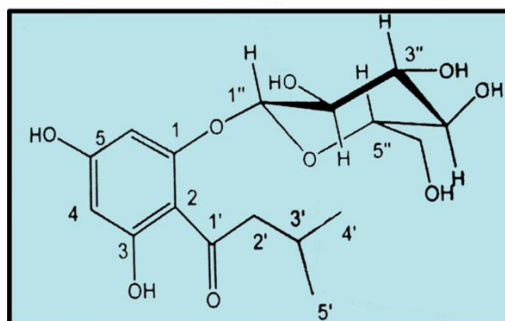
\beta -D-glucopyranoside
